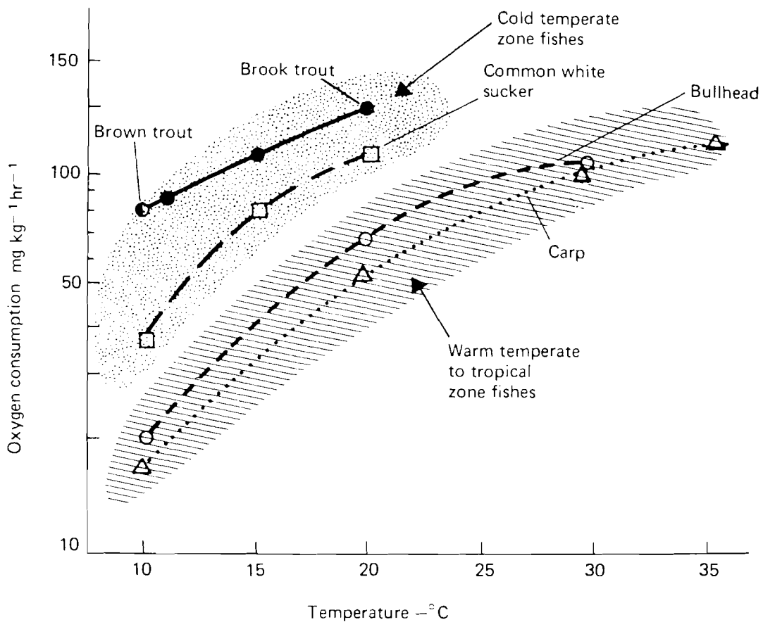
Figure 12 A comparison between the standard metabolic rate (SMR), expressed as oxygen consumption rate, of fishes that have evolved in different latitudinal (climatic) regions. Note that fishes typical of cold waters have higher SMRs than fishes typical of warmer waters (McFarland et al. 1979).
