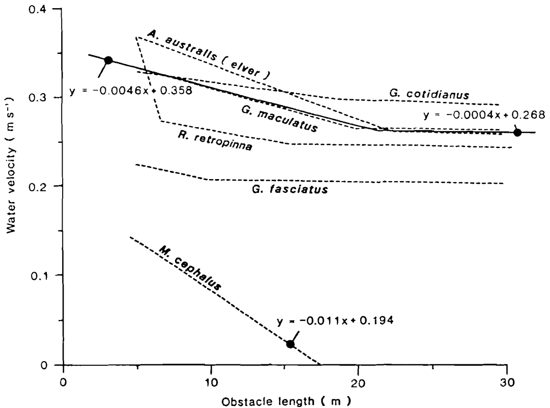
Figure 9 Sustained swimming velocities for shortfinned eel elvers ( Anguilla australis ), inanga ( Galaxias maculatus ), banded kokopu ( G. fasciatus ), common smelt ( Retropinna retropinna ), grey mullet ( Mugil cephalus ), and the common bully ( Gobiomorphus cotidianus ) (from Mitchell 1989).
